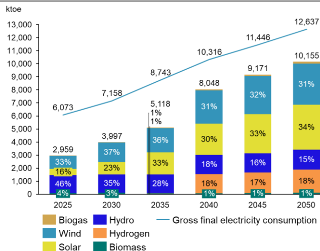
Figure 22. RES evolution by fuel in gross final electricity consumption
