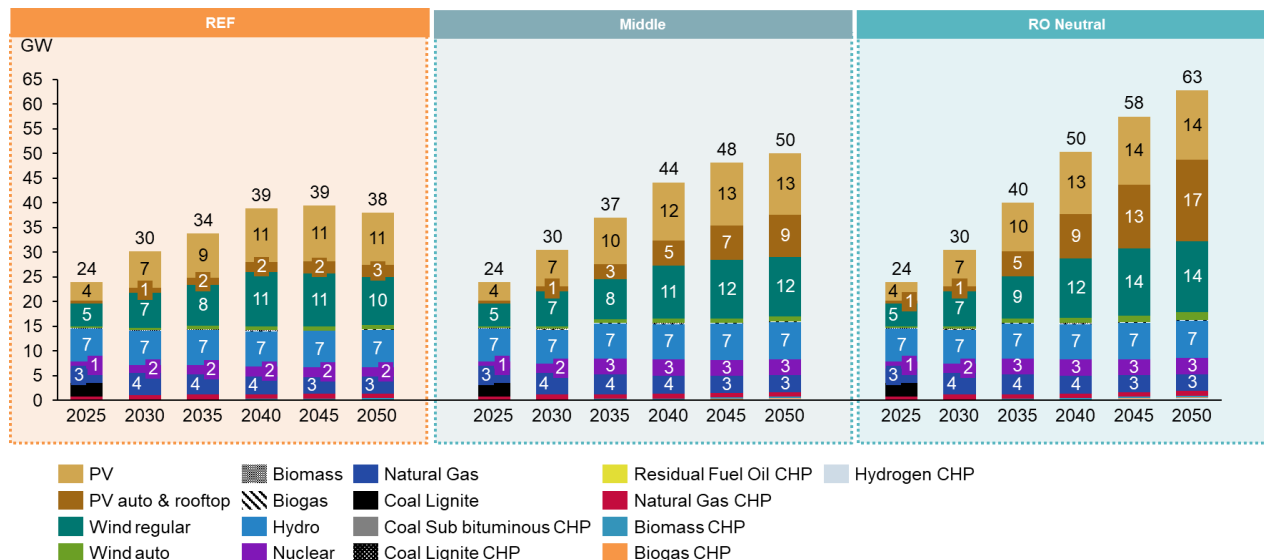
Figure 35. Installed capacity by source – REF, Middle and Romania Neutral scenarios
