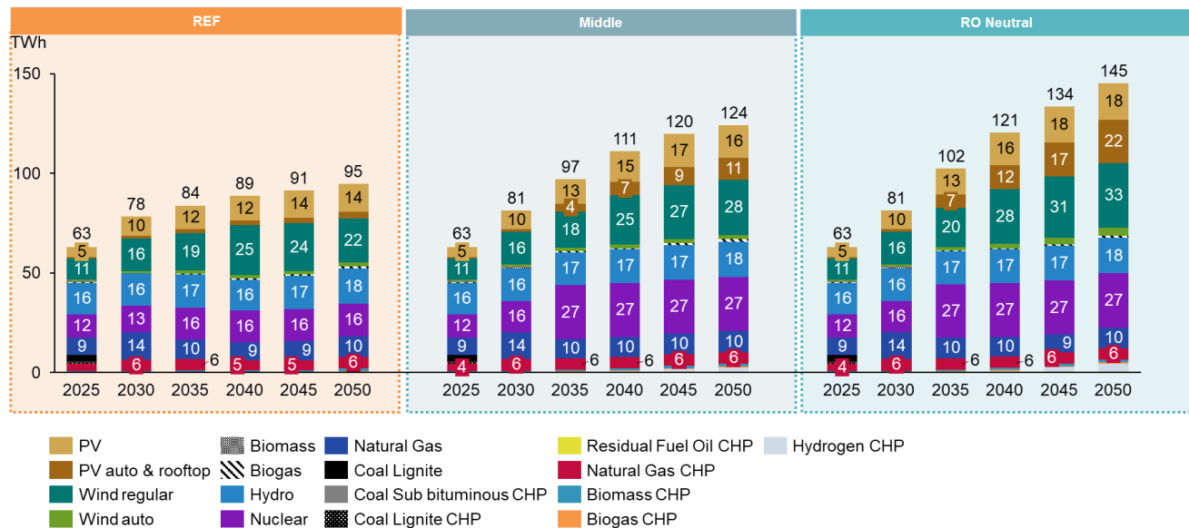
Figure 34. Electricity generation by source – REF, Middle and Romania Neutral scenarios
