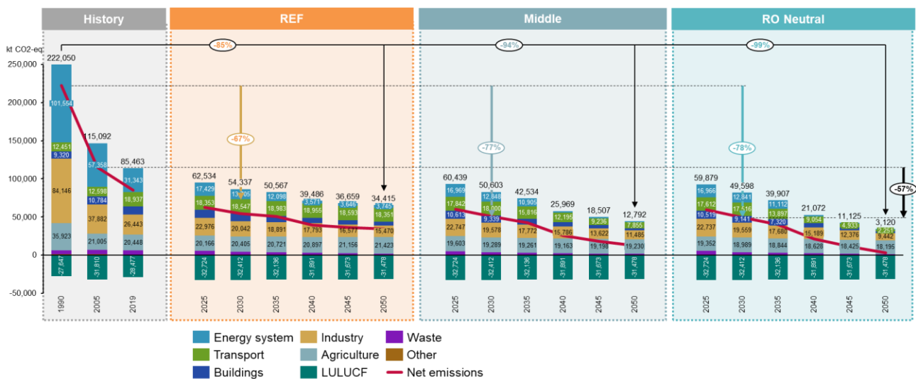
Figure 10. Decarbonization pathways until 2050 by sectors – REF, Middle and Romania Neutral scenarios
