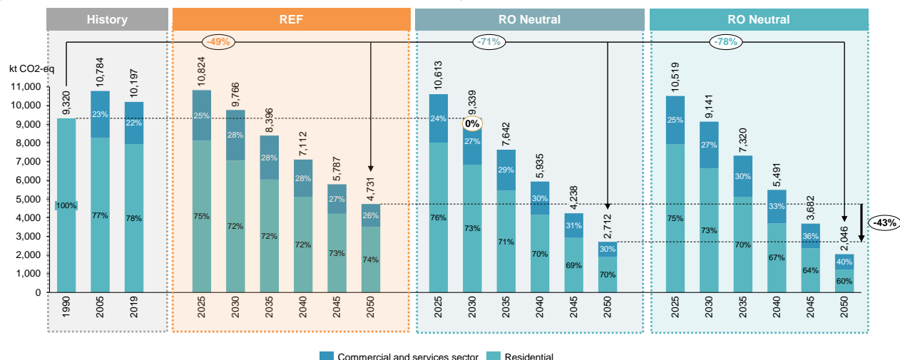
Figure 41. Trajectory of emissions by source in the Buildings sector – REF, Middle and Romania Neutral scenario
