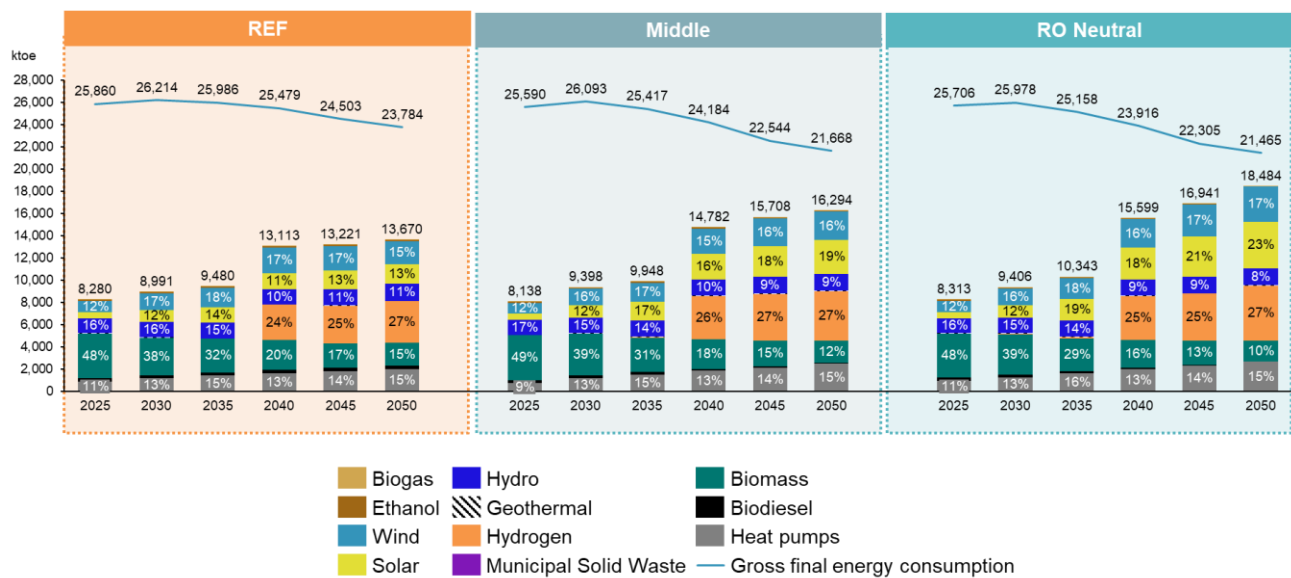
Figure 17. RES share evolution in gross final energy consumption by fuels – REF, Middle and Romania Neutral scenarios
