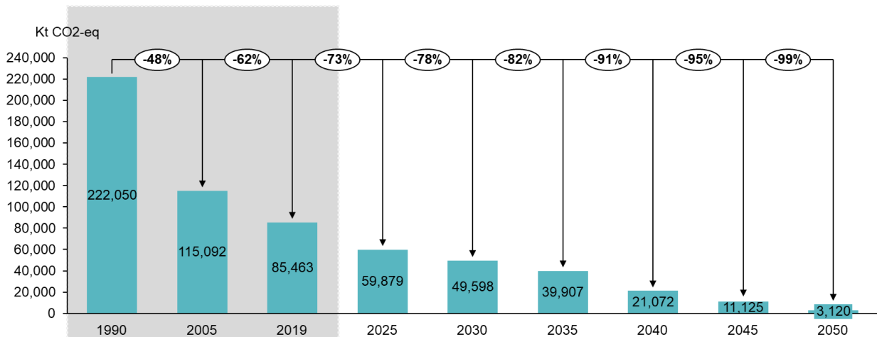
Figure 14. National target for net emissions and indicative milestones by 2050 (Romania Neutral scenario)
