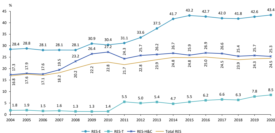
Figure 15. RES share evolution in gross final energy consumption/transport/electricity/ heating and cooling
