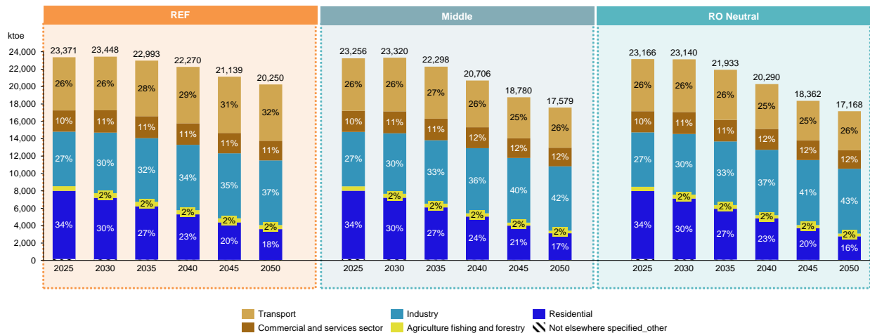
Figure 27. Final energy consumption by sectors – REF, Middle and Romania Neutral
