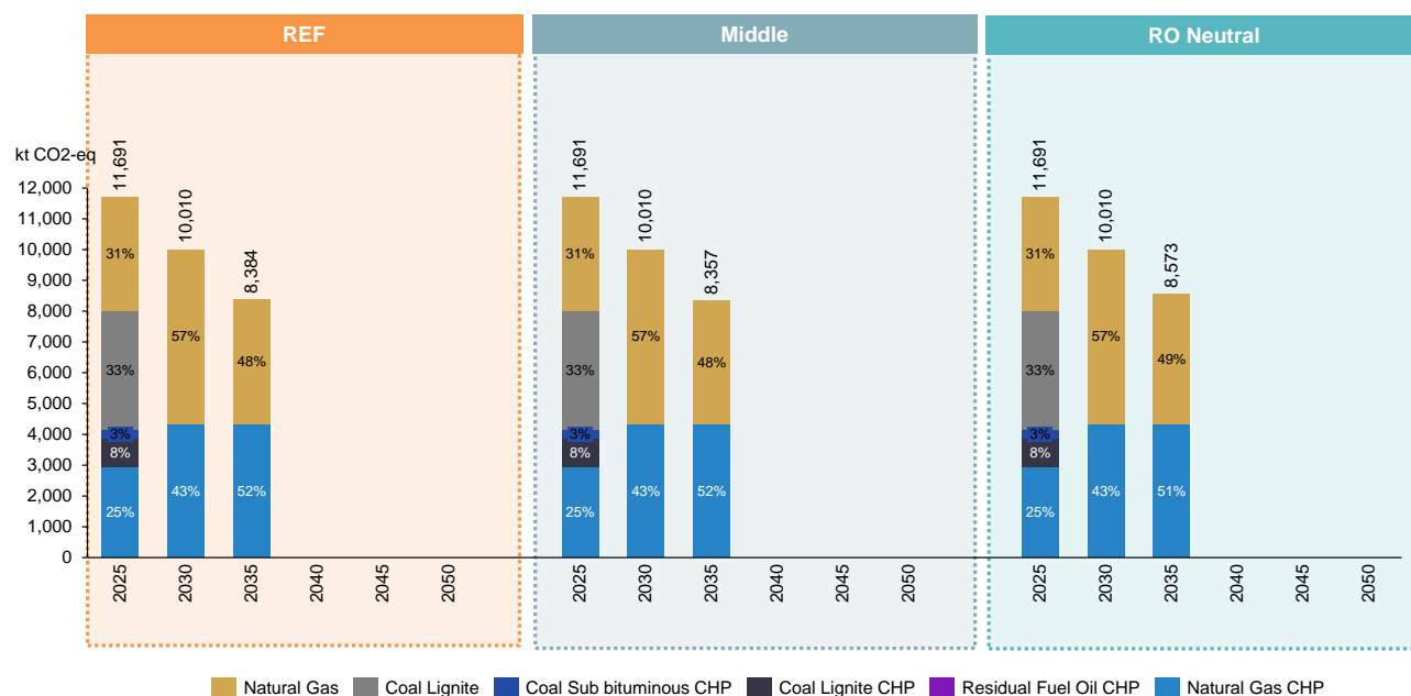
Figure 30. Trajectory of emissions by source in the Electricity generation sector – REF, Middle and Romania Neutral scenario
