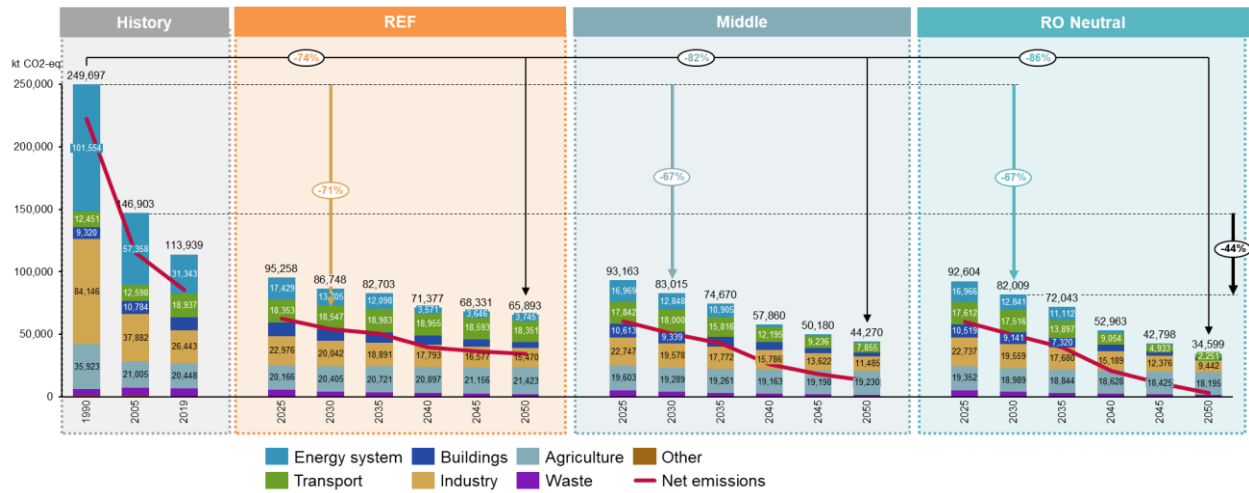
Figure 12. Summary of decarbonization goals of net emissions in 2030 and 2050 – REF, Middle and Romania Neutral scenarios (ktCO2-eq)
