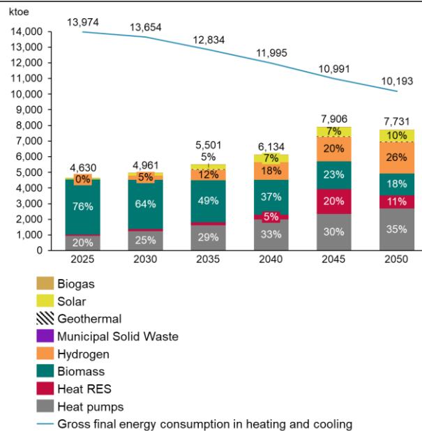
Figure 23. RES evolution by fuel in gross final energy consumption in heating & cooling
